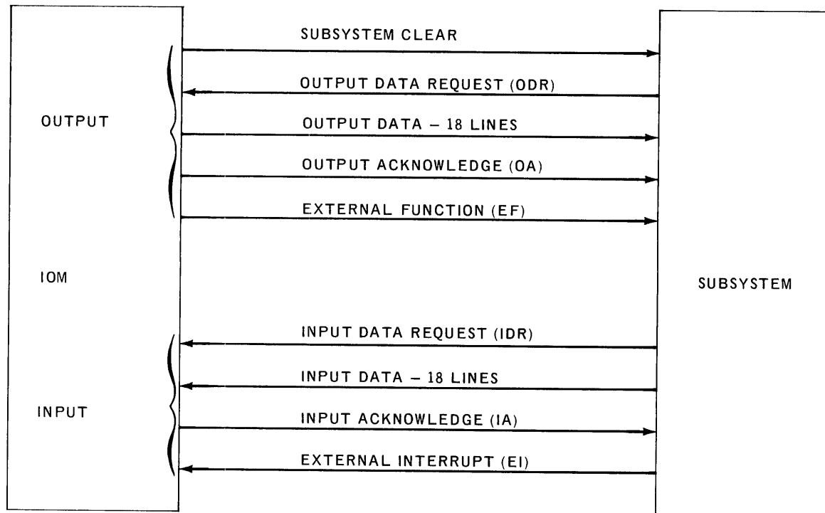
Figure 4-1. One I/O Channel
