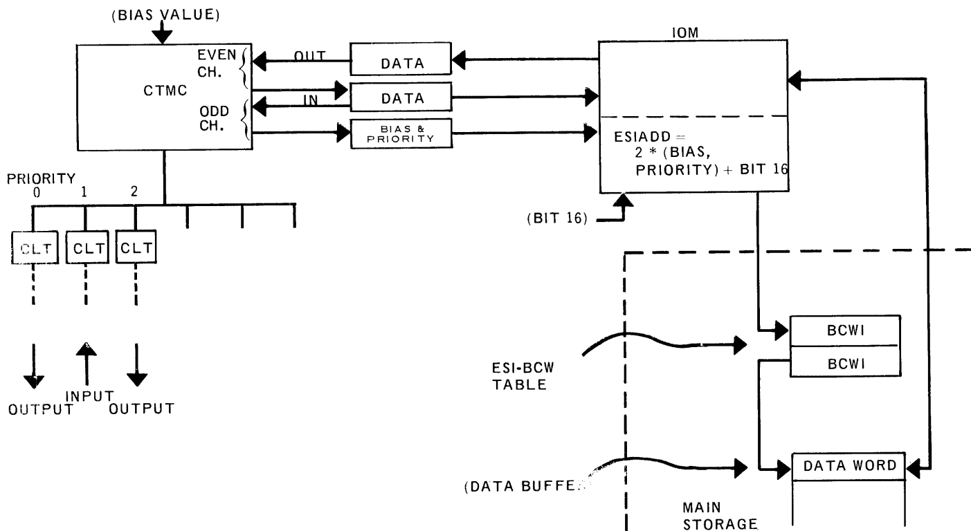
Figure 4-2. ESI Data Transmission
